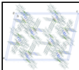
Fig. 2. A view of the packing of the title compound. The red dashed lines represent C32—H32(pyridyl)⋯N2 i (pyridyl) interactions that connect the molecules along the b axis (symmetry code: i : - x +1, - y , - z ). The other interactions are omitted for clarity. Color codes: Green P, Blue N, Gray C.
