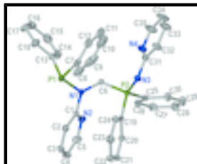
Fig. 1. The atom-numbering scheme of the title compound. Displacement ellipsoids are drawn at the 30% probability level and H atoms are omitted for clarity.
